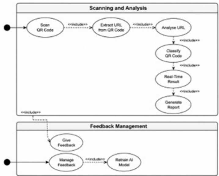
Figure 2 – Use case diagram of the aQRace system
