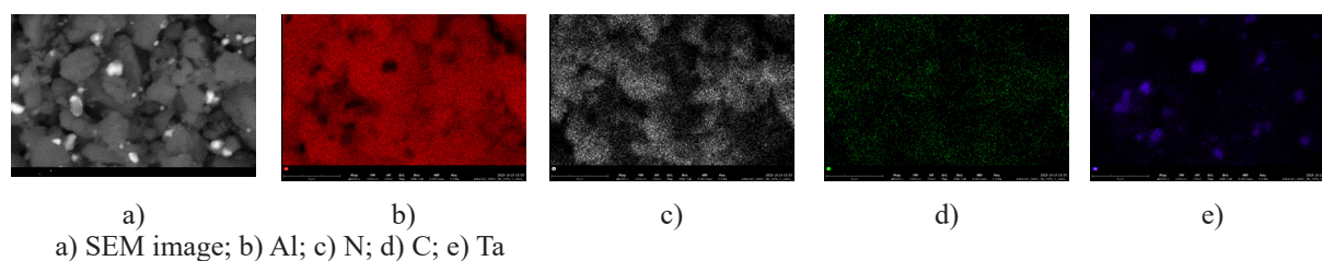
Figure 2 – SEM micrograph and corresponding EDS elemental maps of the (1-x)\text{AlN}-x\text{TaC} composite with x = 0.10
