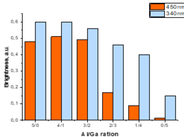
Figure 7 – Relative luminance Y_3Al_xGa_{5-x}O_{12}:Ce ceramic powders as a function of Al/Ga ratio under \lambda_{ex} = 340 nm (n-UV) and \lambda_{ex} = 450 nm excitation, normalised to the SDL 4000 standard
