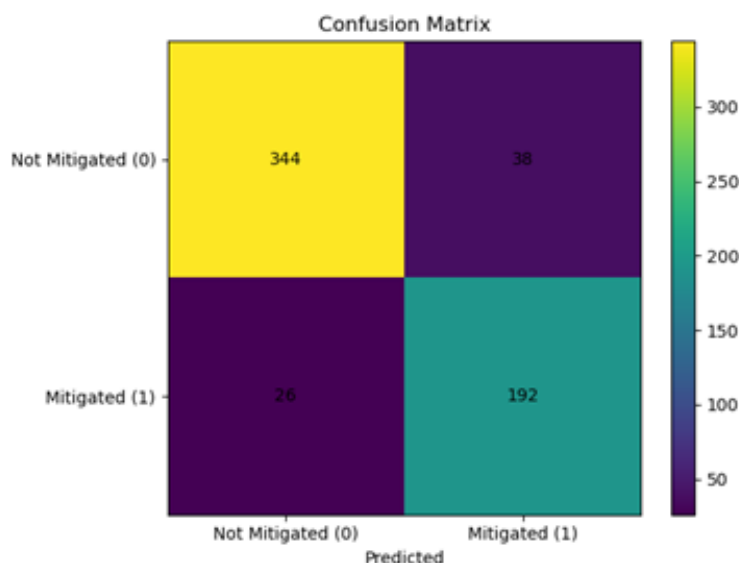
Figure 2 – Confusion matrix of the Random Forest model
