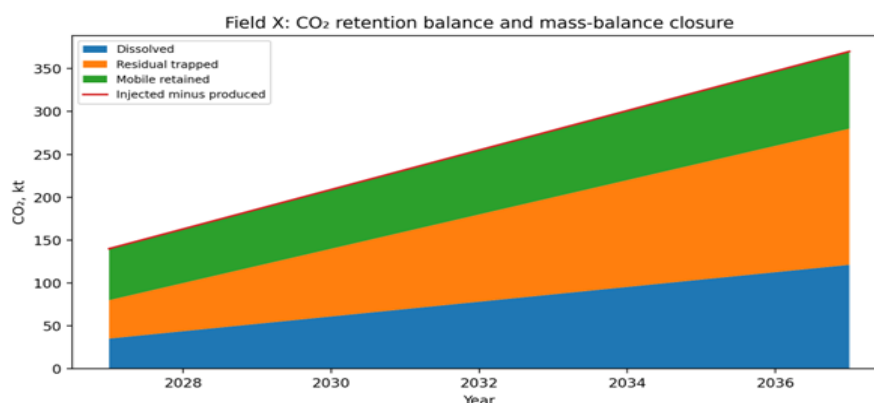
Figure 8 – Field X CO 2 retention balance. Dissolved, residual-trapped and mobile retained CO 2 sum exactly to injected minus produced CO 2 for the reported diagnostic cases
